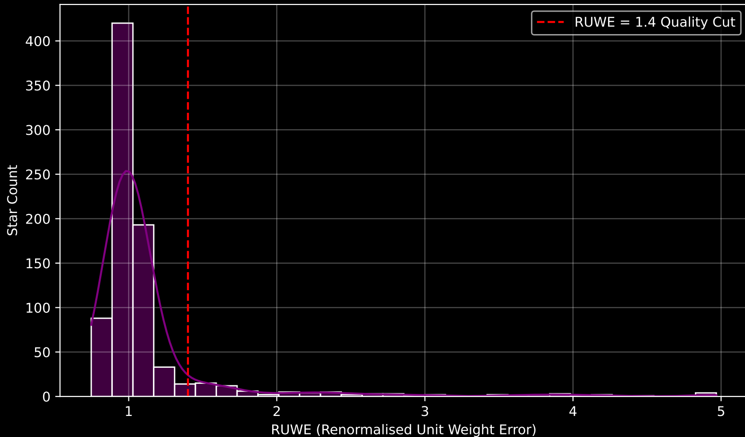
GAPOGEE DR17 Field [K16_075+11] RUWE Distribution (n= 824)
