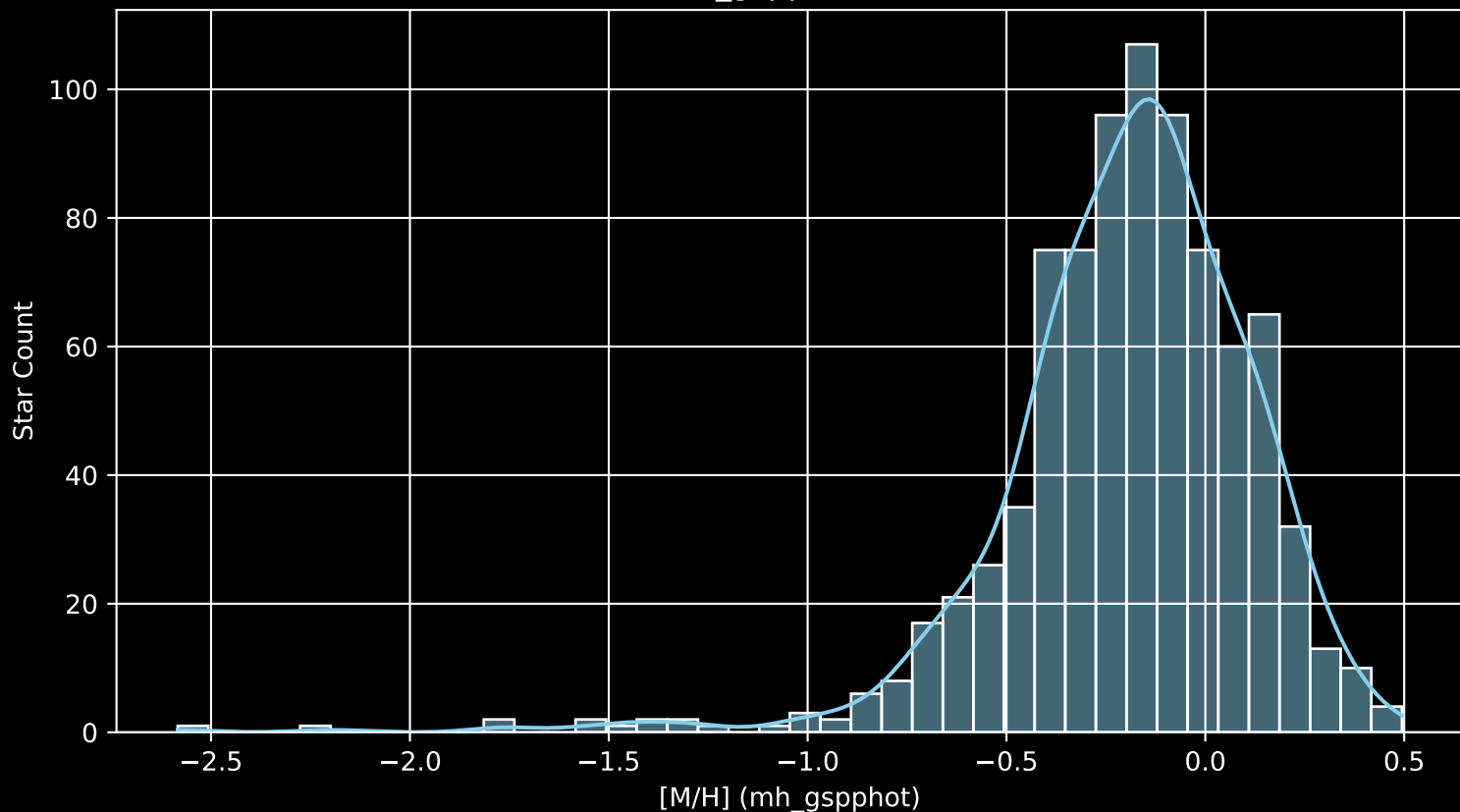
APOGEE DR17 Field: [K16_075+11] [M/H] (mh_gspphot) (n= 839)
