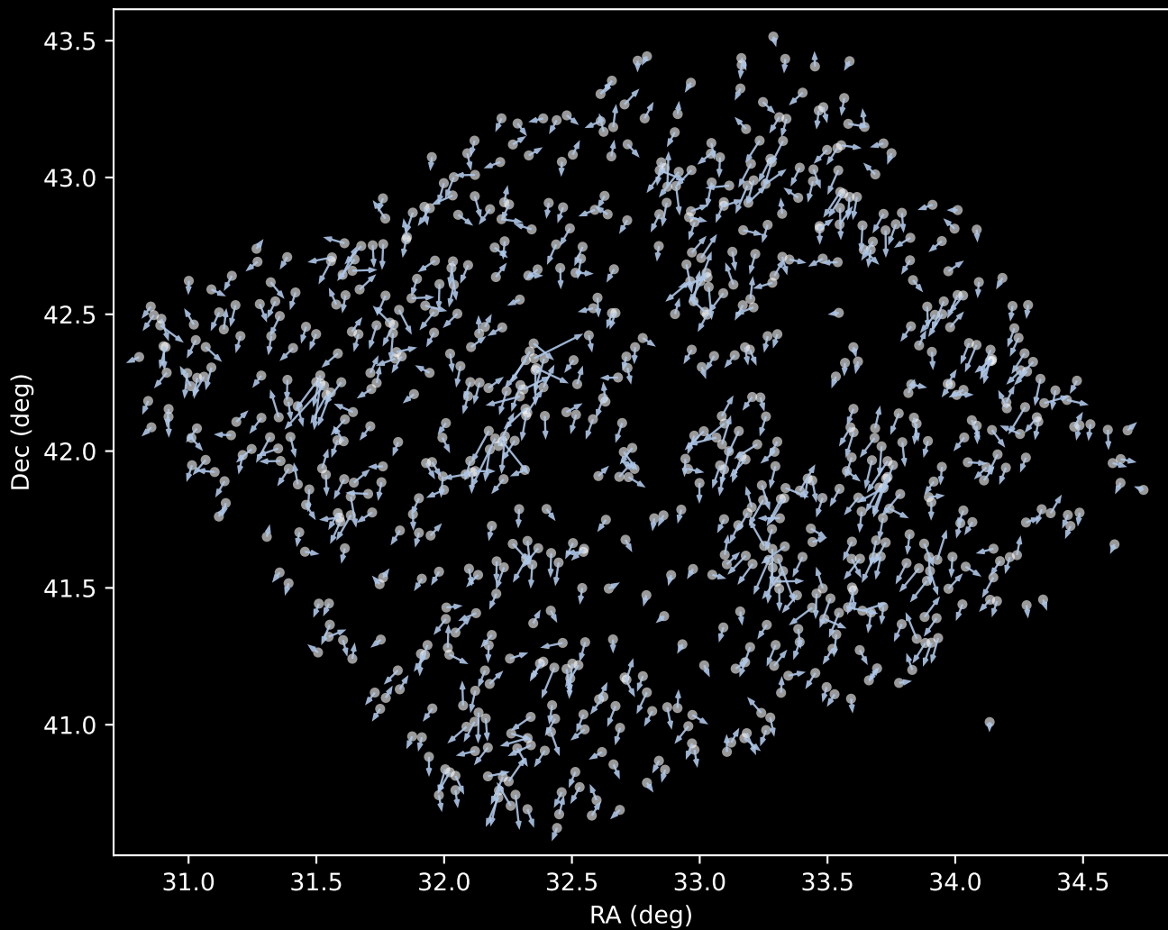
APOGEE DR17 Cluster 1 Proper Motion Vectors (n=772)
