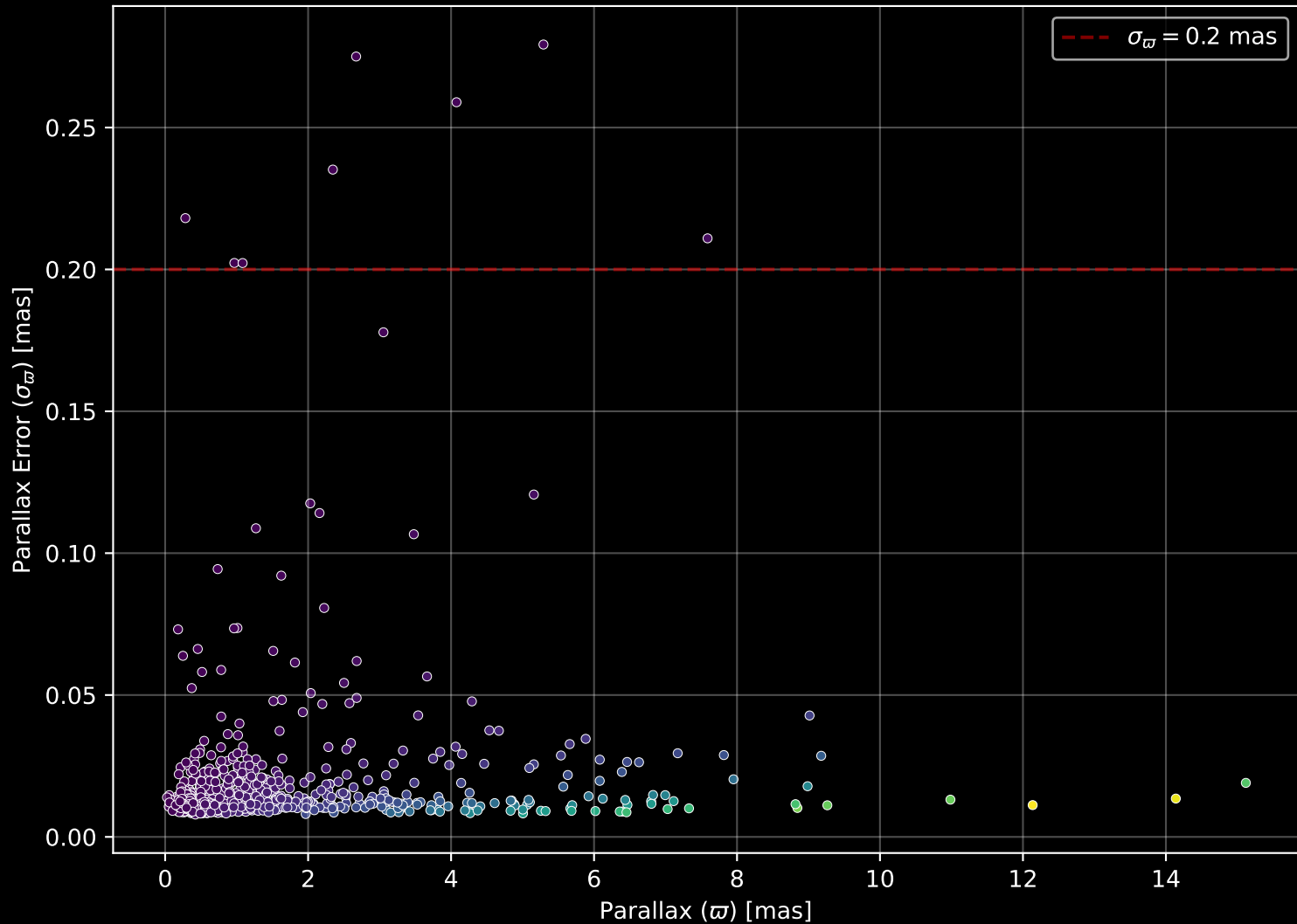
APOGEE DR17 Field: [K16_075+11] Parallax Quality (n= 846)
