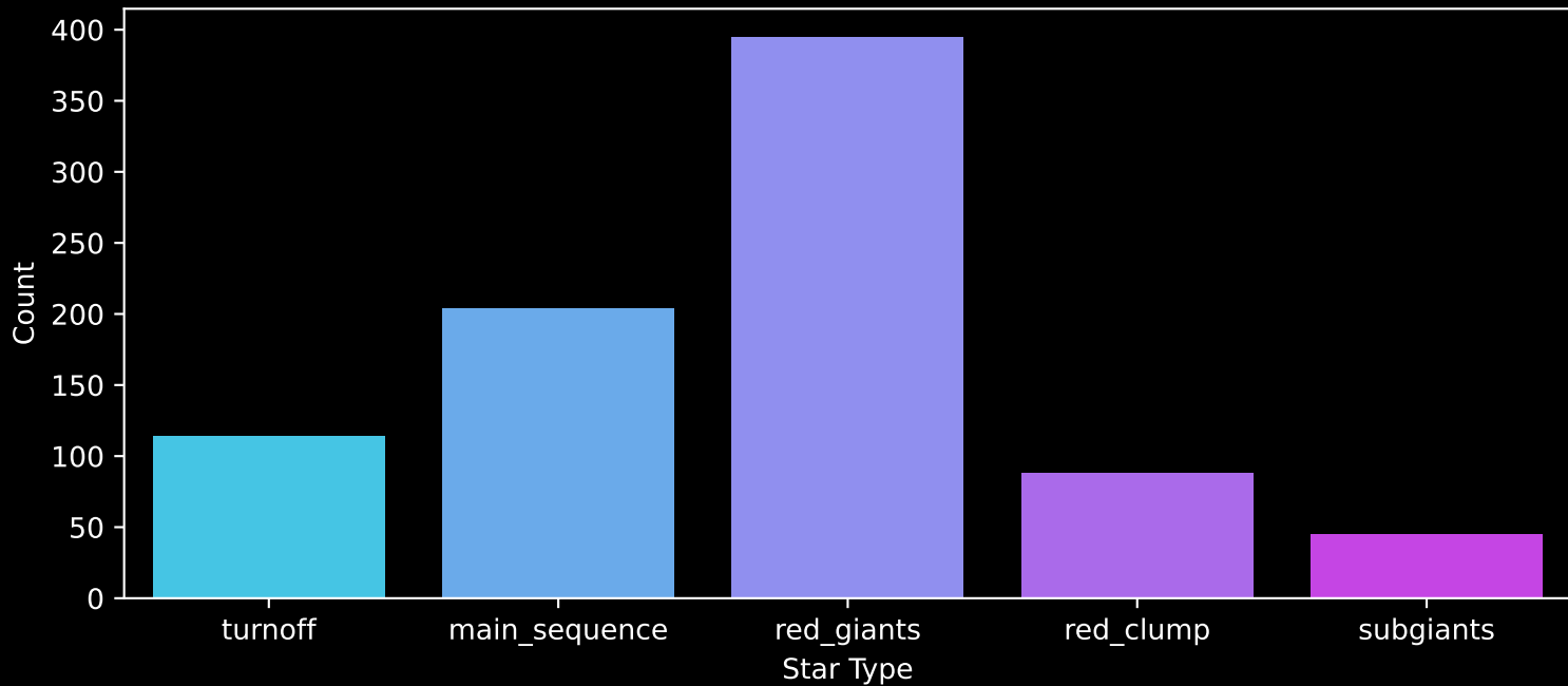
APOGEE DR17 Field: [K16_075+11] Count plot of Star Type
