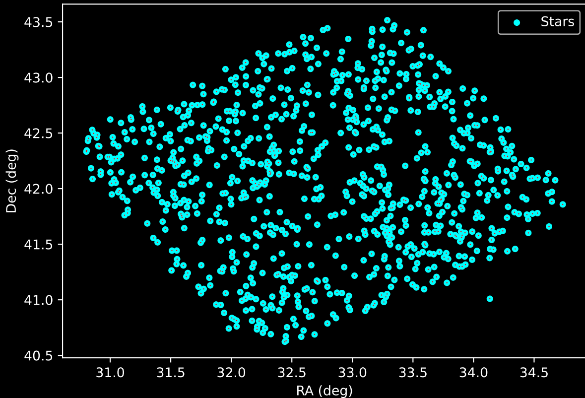
APOGEE DR17 Field: [K16_075+11] Proper Motion Vectors for Gaia Star Field (n= 846)
