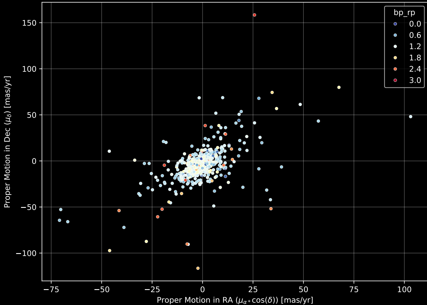
APOGEE DR17 Field: [K16_075+11] Proper Motion Diagram (n= 846)
